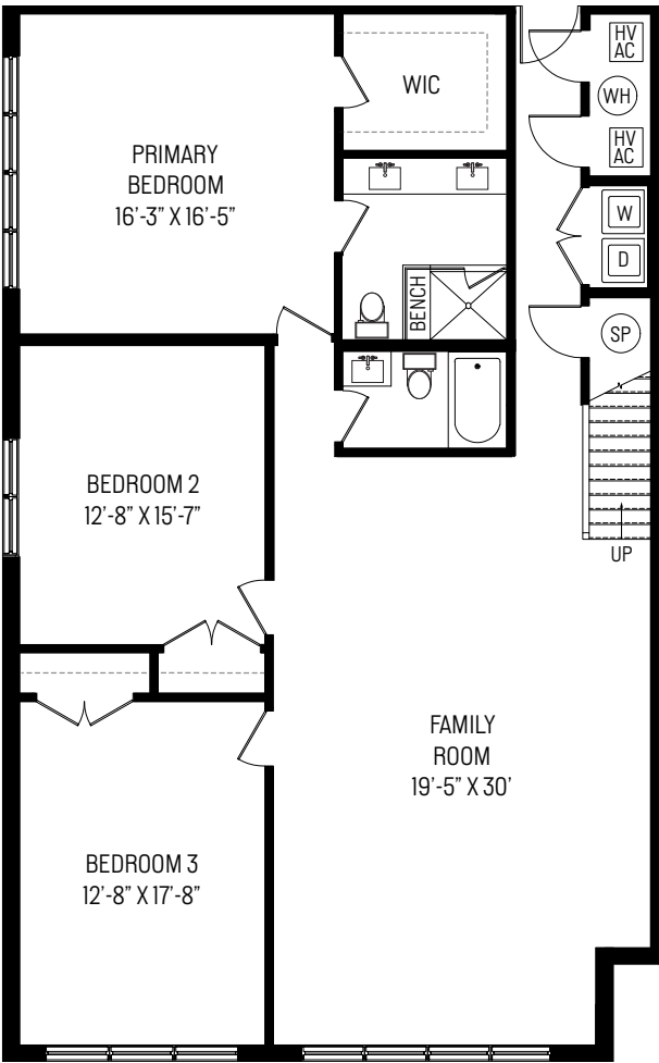
LOWER LEVEL
