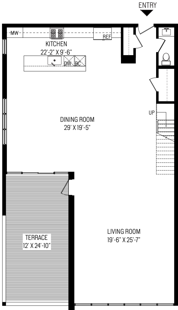
MAIN LEVEL
