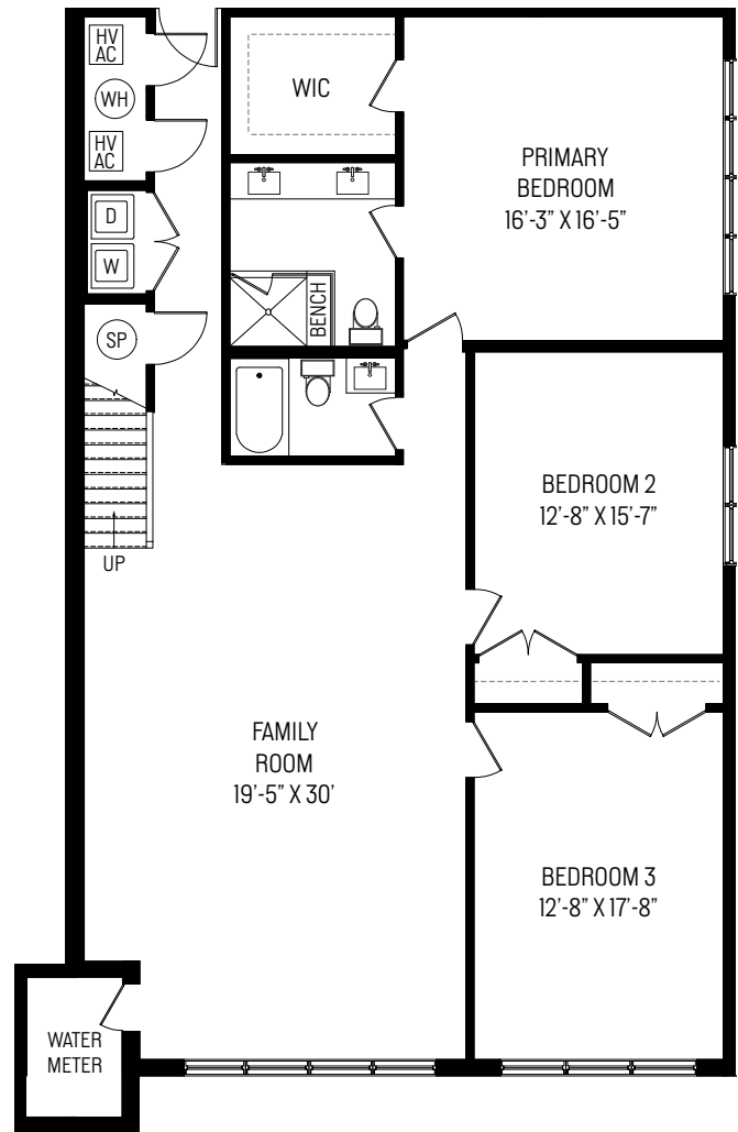
LOWER LEVEL
