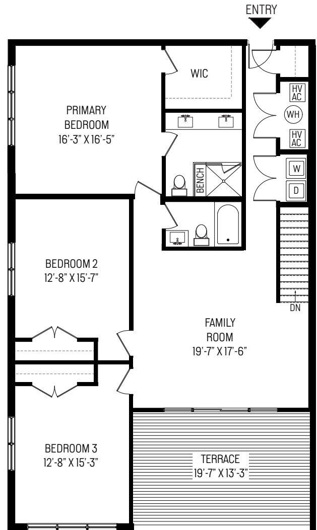
UPPER LEVEL
