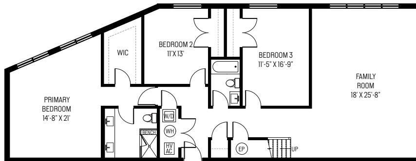
LOWER LEVEL
