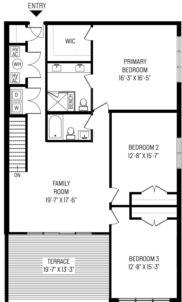
UPPER LEVEL
