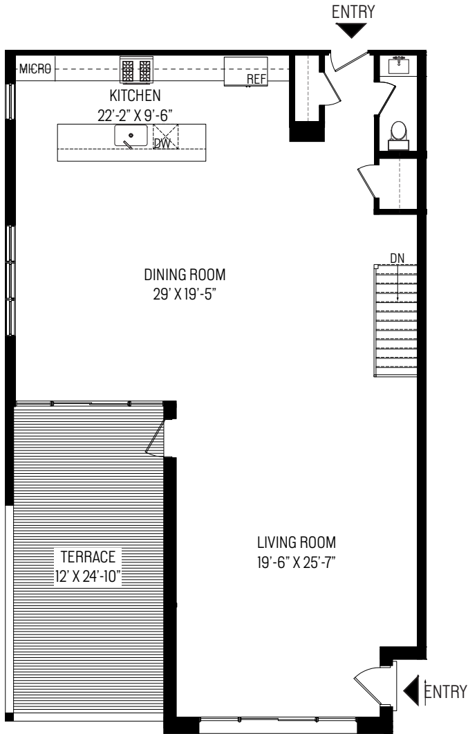
MAIN LEVEL
