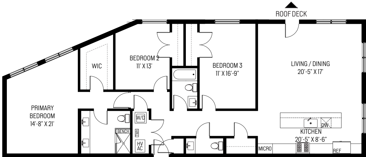
ROOF DECK
