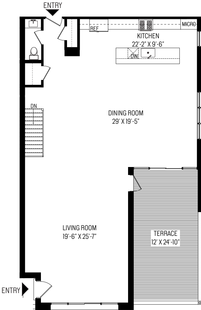
MAIN LEVEL
